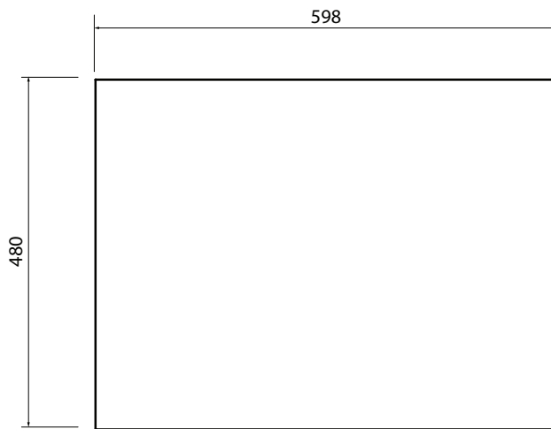
Stone Quartz Top 598 x 480 x 20mm
