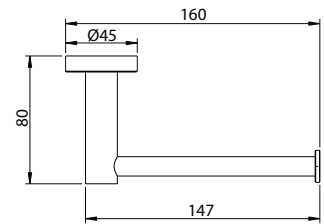
Toilet Roll Holder IN-P2504-BG
